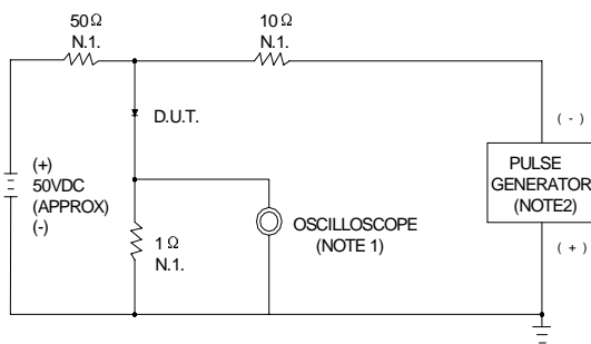
FIG.5-REVERSE RECOVERY TIME CHARACTERISTIC AND TEST CIRCUIT DIAGRAM
